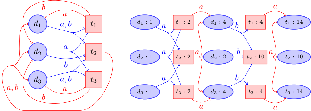
Figure 1: Left. Arena of our running example of an entropy game. Circles are states of the Despot while squares are states of the Tribune. At each move, the player has to choose between actions a and b , the outcome of which may sometimes be non-deterministic (e.g. when Despot plays a in state d_2 , the next state may non-deterministically be either t_1 or t_3 ). Right. A finite play on this arena. Despot plays ab (whatever his opponent does) while Tribune plays aa . We only give, for each step, the number of words that end up in each state controlled by the active player.
