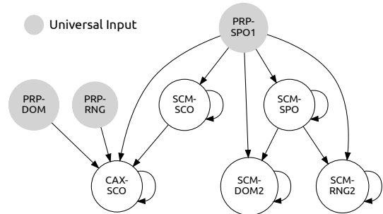
Figure 2: Rules dependency graph for \rho\text{df}
