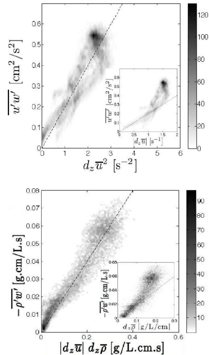
FIG. 3: Two dimensional histograms representing the correlation between turbulent stresses and mean gradients. Grayscale represents a number of entries in the histogram. (a) Momentum flux \overline{u'w'} vs square of vertical velocity gradient \partial_z \bar{u}^2 ; (b) density flux \overline{\rho'w'} vs product of vertical velocity and density gradient \partial_z \bar{u} \partial_z \bar{\rho} . The insets show a test of the linear assumption: \overline{u'w'} vs \partial_z \bar{u} in (a) and \overline{\rho'w'} vs \partial_z \bar{\rho} in (b). The respective slopes indicated by dashed lines yield respectively L_m^2 and L_\rho^2 for the main plots and \nu_T and \gamma_T for the insets.
