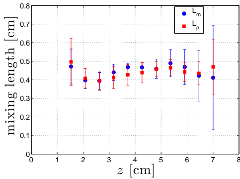
FIG. 4: (Color Online) Mixing lengths L_m ( \bullet ) and L_\rho ( \square ) vs distance z from the plane. The error bars correspond to the standard deviation computed from the average along x .
