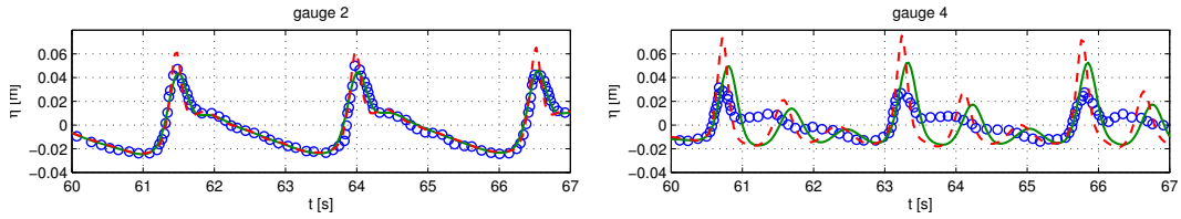
Figure 23: Propagation over a submerged bar, case (b); data in gauge 2 (left) and gauge 4 (right): experimental data [3] ( \circ ), BNA model ( \text{—} ), BN model ( \text{- -} ).
