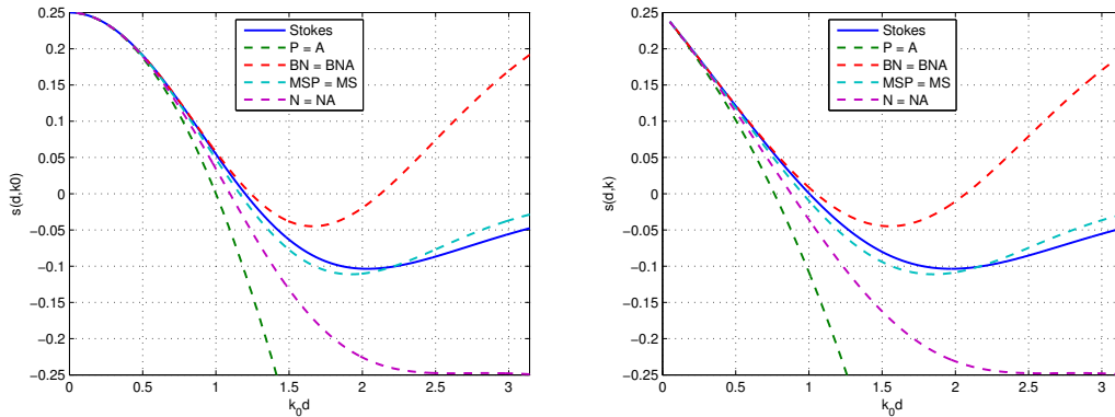
Figure 4: Linear shoaling: representation of the linear shoaling coefficient s of the several BT models defined by (39). On the left is sketched s(h(x), k_0) , thus computing the values of s using the initial wavenumber of the signal k_0 . On the right, instead, the variation of k along the domain is considered in the computation of the shoaling coefficient, thus: s(h(x), k(x)) .
