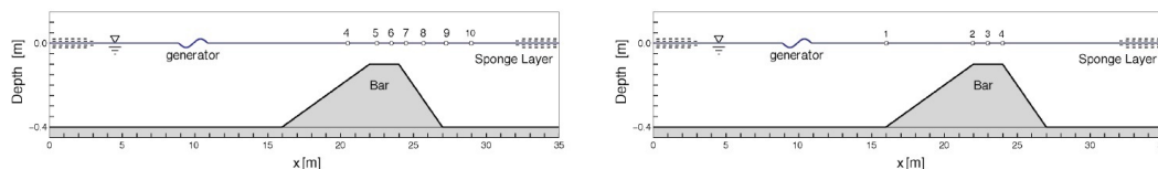
Figure 14: Periodic wave propagation over a submerged bar: sketch of the computational configuration and of the gauges position; case (a) on the left, case (b) on the right.
