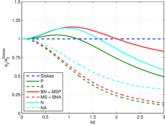
Figure 3: Ratio of the second harmonic a_2/a_2^{Stokes} for the models considered. Continuous line : amplitude-velocity models. Dashed lines : amplitude-velocity models. Refer to figure 2 for the legend.
