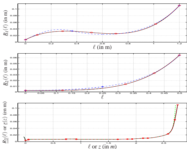
Figure 1: Test profiles \underline{R}_k (-). For \underline{R}_1 and \underline{R}_2 : examples of optimal approximation with N = 2 , N = 4 and N = 6 pieces of pipes (- - + and - - o). Original bore r_3(z) (- - -), \underline{R}_3(\ell) (-) and approximation with N = 11 pieces of pipes (- - o).
