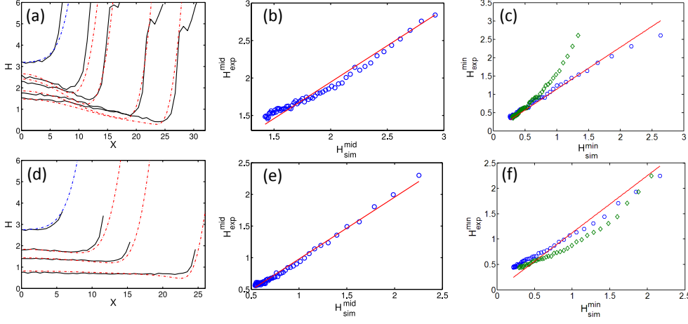
FIGURE 7. (a-d) Experimental thickness profiles (black lines) compared with simulated thickness profiles obtained from integration of equations (4.5) and (4.6) (red dashed lines). The blue dashed line is the initial profile for the simulation, calculated from the corresponding experimental profile in black. Thicknesses are reported in dimensionless units H = h/(R_c(3Ca)^{2/3}) , as a function of the dimensionless position X = x/(R_c(3Ca)^{1/3}) . (b-e) Experimental thickness in the middle of the film as a function of the simulated central thickness, corresponding to X = 0 on figures (a) and (d). (c-f) Experimental minimal thickness as a function of the minimal thickness obtained with our simulation ( \circ ), and as a function of the Frankel's prediction ( \diamond ). The measurements (a-b-c) correspond to the low viscous case (1.3mPa.s) with a radius of curvature of 250 \mu\text{m} and \lambda = 0.02 , and (d-e-f) to the high viscous case (3.4mPa.s) with a radius of curvature of 224 \mu\text{m} and \lambda = 0.07 . Red line corresponds to a linear fit, whose slopes are close to one (0.97, 1.14, 0.98 and 1.13 for (b), (c), (e), (f) respectively). Results are obtained for solution F (top line) and G (bottom line).
