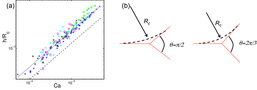
FIGURE 5. (a) Minimal thickness of the film normalized by the radius of curvature of the Plateau border, as a function of the capillary number Ca = \eta V / \gamma . The curve gather measurements for the frame of side 8mm with \eta = 1.4\text{mPa.s} and 240 < R_c < 320\mu\text{m} (x), \eta = 1.4\text{mPa.s} and 160 < R_c < 240\mu\text{m} ( \Delta ), \eta = 1.4\text{mPa.s} and 110 < R_c < 160\mu\text{m} ( \star ), \eta = 2.2\text{mPa.s} and 240 < R_c < 320\mu\text{m} ( \ast ), \eta = 2.2\text{mPa.s} and 110 < R_c < 160\mu\text{m} ( + ), \eta = 3.4\text{mPa.s} and 240 < R_c < 320\mu\text{m} ( \square ), \eta = 5.1\text{mPa.s} and 240 < R_c < 320\mu\text{m} ( \nabla ), and for the frame of side 4mm with \eta = 1.4\text{mPa.s} (o). The dashed line corresponds to Frankel's law h/R_c = 2.68Ca^{2/3} and the straight line corresponds to a fit of the data with h/R_c = 4.5Ca^{2/3} . (b) Scheme representing Plateau border radius of curvature variations due to out-of-equilibrium shape of film assembly, the angle varying between \pi/2 at the beginning of the relaxation process to 2\pi/3 .
