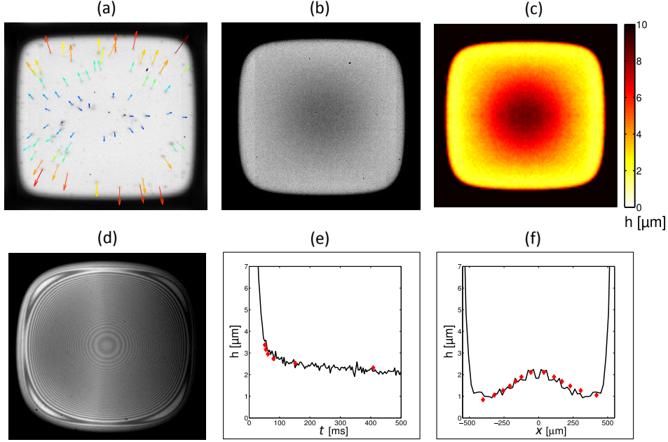
FIGURE 2. (a) Velocity of the particles 13ms after the creation of the fresh film, for a solution of SDS with dye and 40% of glycerol. (b-c) Thickness measurement through light absorption 100ms after the creation of a film of a solution of SDS containing a dye. The light intensity (b) and the corresponding thickness (c) are represented. Thickness bars are in \mu\text{m} . (d) Thickness measurement through monochromatic interferences observed 28ms after the film creation for a solution of SDS with dye and 10% of glycerol. (e) Evolution with time of the thickness at the center of the new film measured by absorption (black line) and interferometry (red dot) for two measurements with comparable evolution of film length, with a mixture of SDS (3g/L), dodecanol (0.3 g/L), dye, and 10% of glycerol. (f) Thickness profile of the same films at t=800\text{ms} .
