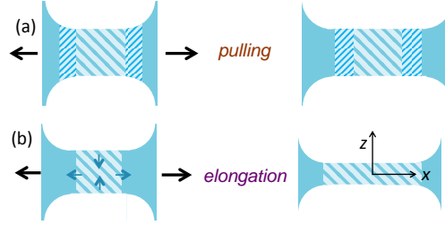
FIGURE 4. Two limit cases of film formation, with the state at t represented on the left, and the state at t + dt represented on the right. The color indicates different volumes of fluid, followed during their deformation and motion. (a) Pulling: The thin film at t (in gray) is not deformed and some of the fluid present in the Plateau border at t goes into the film at t + dt . The velocity in the thin film is 0, so k = 0 . (b) Stretching: There is no volume exchange between the film and the Plateau border. The thin film of length 2L at t (in gray) is stretched at t + dt to reach the length 2L + 2\dot{L}dt . The velocity in the film is V_x = \dot{L}x/L , corresponding to k = 1 . Actual deformation is a combination of these two limit cases, leading to 0 \leq k \leq 1 .
