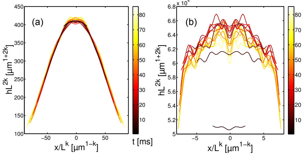
FIGURE 6. (a)-(b) Self-similarity of thickness profiles measured by absorption for solutions of SDS and dye at viscosities of 1.4 (a) and 3.4mPa.s (b) with R_c = 280\mu\text{m} (from figure 3(h) and (i)). k is adjusted to superimpose the thickness profiles, and is here equal to 0.36 and 0.95 for 1.4mPa.s and 3.4mPa.s respectively.
