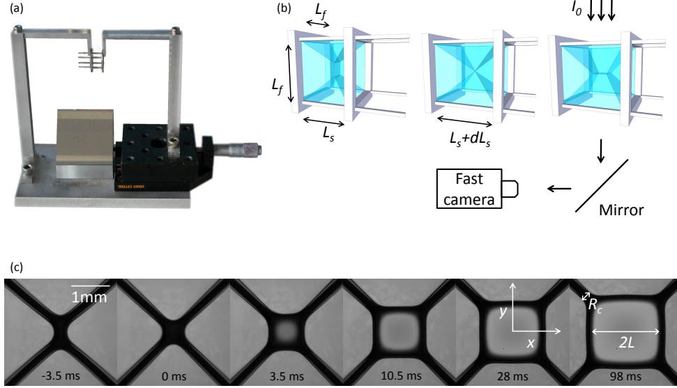
FIGURE 1. (a) Picture of the frame with the micrometric screw and the mirror. (b) Film network created in the frame before the T1 event (left), in the metastable configuration (middle), and at the end of the rearrangement (right). (c) Image sequence of the freshly created film. R_c is the radius of curvature of the Plateau border, and 2L the length of the film.
