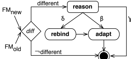
From TABLE I and TABLE II : \delta = \{\text{Add mand. } f; \text{ Remove mand. } f, f \in C; \dots\} \beta = \{\text{Add constraint; Update cardinality; } \dots\} \gamma = \{\text{Remove opt. } f, f \notin C; \dots\}
