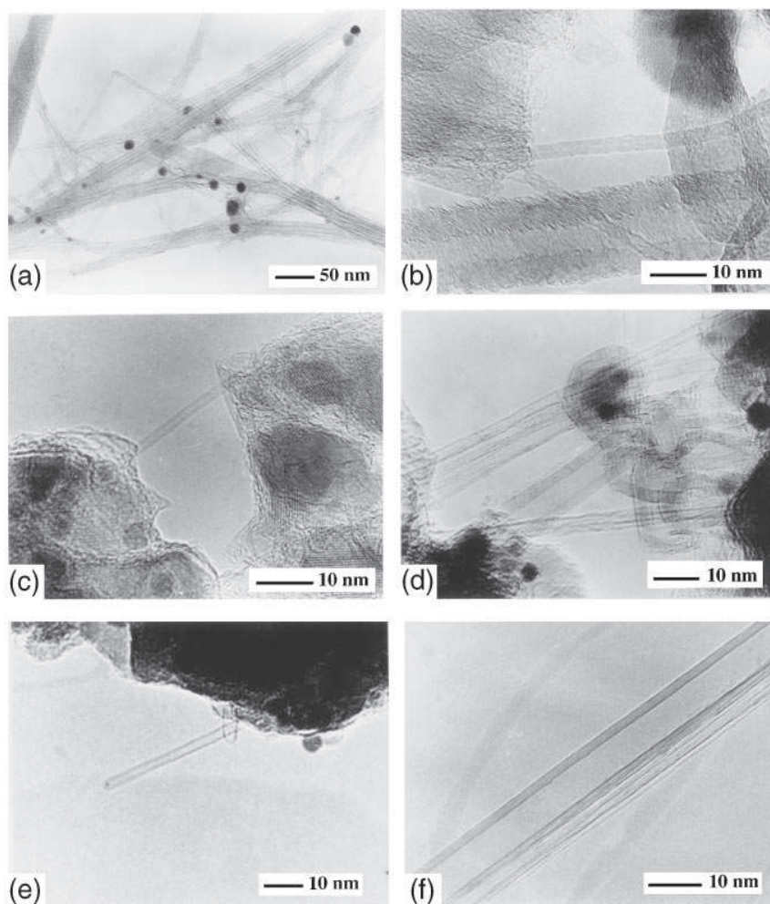
FIG. 9. TEM images of the nanocomposite powders subjected to H_2-CH_4 treatment at 1070 °C: (a) Fe0.2; (b) Fe0.2; (c) Co0.1; (d) Co0.2; (e) Ni0.2; (f) Ni0.2.
