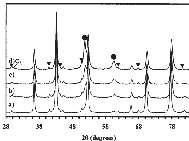
FIG. 5. XRD patterns of the Co-containing nanocomposite powders after treatment with \text{H}_2 - \text{CH}_4 at 1070 °C ( \text{Co}_x ): (a) x = 0.1 ; (b) x = 0.2 ; (c) x = 0.3 ; (d) x = 0.4 . (●) \epsilon -Co; (▼) \alpha - \text{Al}_2\text{O}_3 contamination from the attrition balls. Cg corresponds to d_{002} in multiwall nanotubes and/or in graphite; other peaks: spinel matrix.
