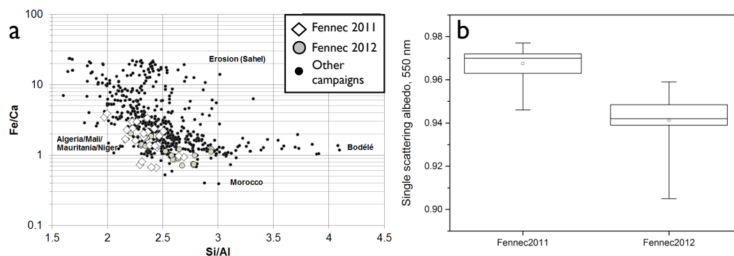
Figure 5. (a) Scatter plot of the elemental Fe / Ca vs. the Si / Al ratios for the Fenec 2011 and 2012 samples compared to samples collected during the AMMA, DODO and GERBILS campaigns (Formenti et al., 2014). Indications of the source regions according to the values of those tracers are also given. (b) Box plot of SSAs at 550 nm measured during Fenec 2011 and 2012 for horizontal runs corresponding to filter samples taken. SSAs are calculated from scattering measured by the nephelometer and absorption measured by the PSAP on the BAe146 mounted behind Rosemount inlets, and therefore represent accumulation mode only. Box lines represent the median and interquartile range, whiskers represent the minimum and maximum values and the squares represent the mean.
