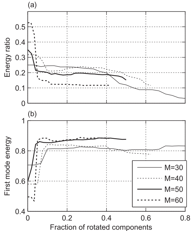
FIG. 4. M-SSA analysis of the SOI and NAO indices, as a function of the relative number S(DM)^{-1} of rotated EOFs and for different values of the window length M ; here D = 2 is fixed. (a) Energy ratio \varepsilon of the leading 7.8-yr oscillatory mode and (b) the unimodality index of the corresponding RCs.
