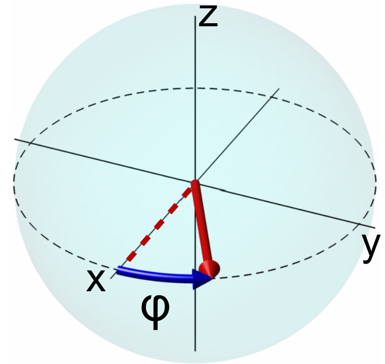
Dephasing
