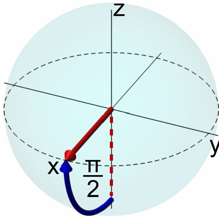
Superposition state
