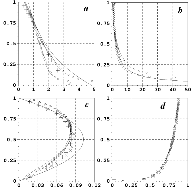
Figure 11. Open-channel turbulent steady flow. Vertical distributions of k / u_*^2 (a), \epsilon H / u_*^3 (b), \nu_T / Hu_* (c) and axial velocity in m/s (d) versus non-dimensional distance to the bed. Present SPH method with \circ EARSM and \diamond linear k - \epsilon model; — semi-empirical [20]; \times experimental [20]; + finite elements k - \epsilon [21].
