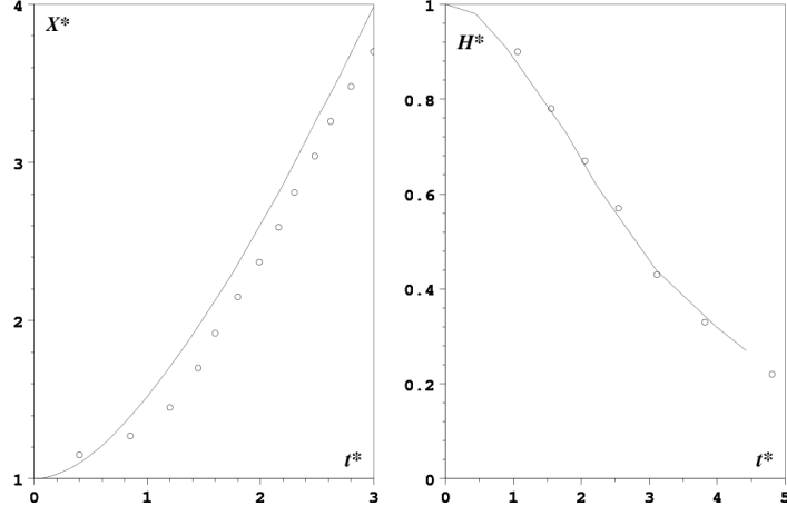
Figure 10. Collapse of a water column in a tank simulated with the present SPH k - \varepsilon model (solid lines). Non-dimensional maximum x -position X^* = X/a and water depth H^* = H/(2a) versus non-dimensional time t^* = t(a/2g)^{1/2} ( a is the initial column width). Validation with experiments (circles) from [22].
