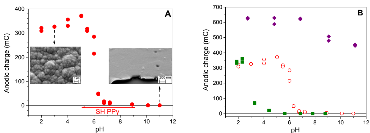
Figure 7: Anodic charge vs. pH of the Py solution after 600 s of polarization at 0.78 \text{ V/SCE} . Electrolyte: A: 0.15 \text{ M Py} + 0.2 \text{ M K}_2\text{HPO}_4 + 10^{-3} \text{ M LiClO}_4 \pm \text{H}_3\text{PO}_4 or \text{KOH} to adjust the pH (initial pH = 8.9 ); B: ( \circ ) same as A ; ( \blacklozenge ) 0.15 \text{ M Py} + 0.2 \text{ M LiClO}_4 ; ( \blacksquare ) 0.15 \text{ M Py} + 0.2 \text{ M K}_2\text{HPO}_4 . Inset A: SEM images of the films obtained at pH 3 and 11 (Substrate: Au/mica). Scale bars: 1 \mu\text{m} (pH 3), 200 \text{ nm} (pH 11). SH PPy: superhydrophilic PPy film.
