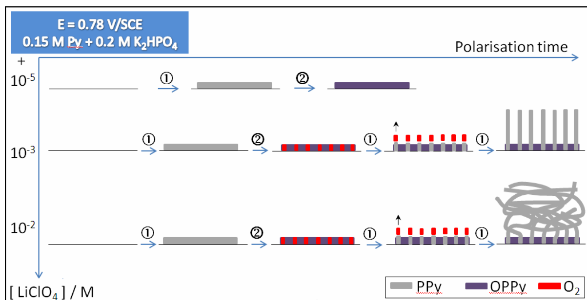
Figure 6: Schematic model showing the process which takes place depending on the perchlorate concentration of a 0.15 M Py + 0.2 M \text{K}_2\text{HPO}_4 solution on the electrode polarized at 0.78 V/SCE. ①: Py oxidation ; ②: water oxidation ( \text{OH}^\bullet and/or \text{O}_2 production).
