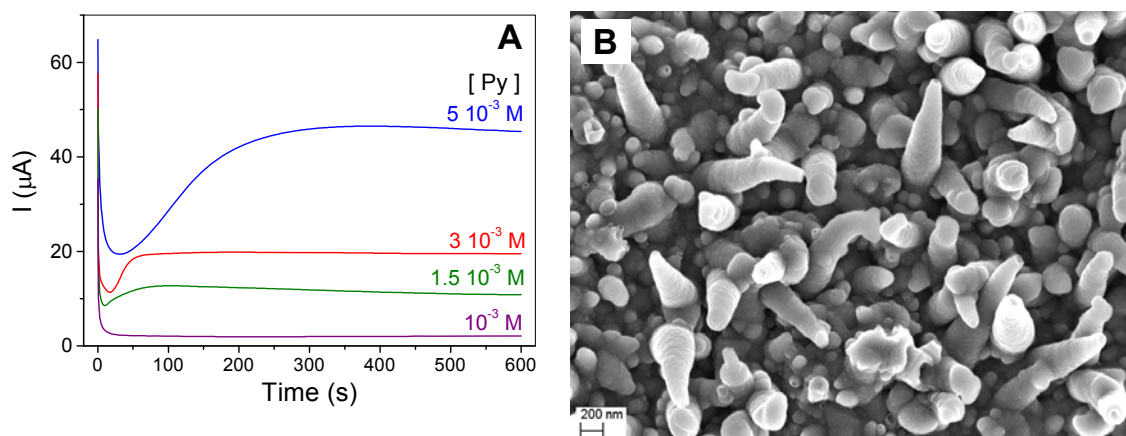
Figure 8: A: Current density vs. time a Pt electrode ( S = 0.07 \text{ cm}^2 ) polarized at 0.75 V/SCE in 0.2 M \text{LiClO}_4 + Py aqueous solution. Py concentrations are indicated in the graph. Anodic charge: 1.3 mC (1 mM) ; 7 mC (1.5 mM) ; 11.5 mC (3 mM) ; 24.3 mC (5 mM). B: SEM image of a PPy film electrogenerated in 5 \cdot 10^{-3} M Py + 0.2 M \text{LiClO}_4 aqueous solution at 0.75 V/SCE for 300s. Scale bar: 200 nm.
