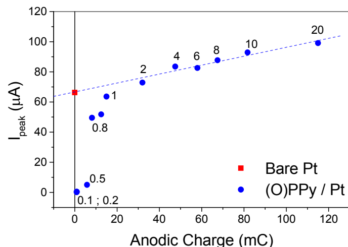
Figure 4: Anodic current peak in 10^{-2} M \text{Fe}(\text{CN})_6^{4-/3-} + 0.5 M KCl aqueous solution vs. the anodic charge due to (O)PPy film electrogeneration at 0.78V/SCE for 600 s in \text{LiClO}_4 (concentrations in mM are indicated in the graph) + 0.2 M \text{K}_2\text{HPO}_4 + 0.15 M Py solution. Data are from Fig. 3.
