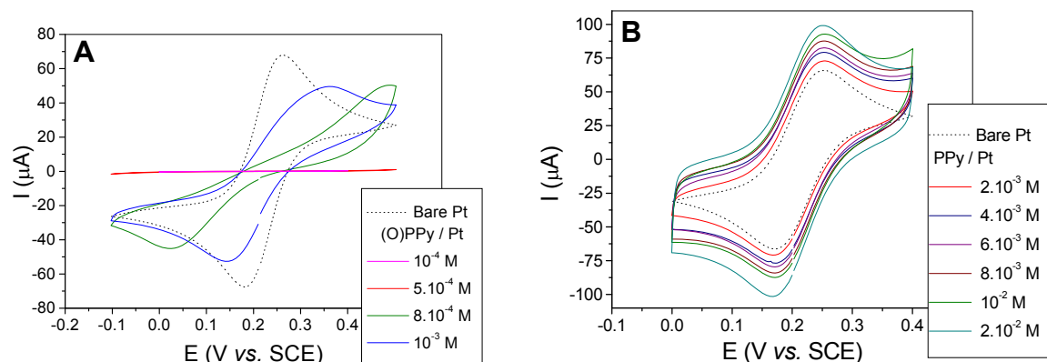
Figure 3: Cyclic voltammograms at a Pt electrode coated with a polypyrrole film obtained under potentiostatic conditions (0.78 V/SCE) in 0.15 M Py + 0.2 M \text{K}_2\text{HPO}_4 + \text{LiClO}_4 aqueous solution. \text{LiClO}_4 concentrations are indicated in the graph (A: 10^{-4} to 10^{-3} M ; B: 2 \cdot 10^{-3} M to 2 \cdot 10^{-2} M). Electrolyte: 10^{-2} M \text{Fe}(\text{CN})_6^{4-/3-} + 0.5 M KCl. Potential scan rate : 10 \text{ mV s}^{-1} .
