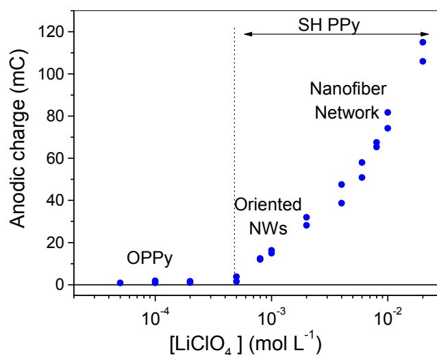
Figure 1: Anodic charge vs. perchlorate concentration of the Py solution. Charge passes through a Pt electrode polarized at 0.78V/SCE for 600 s. Electrolyte: LiClO 4 + 0.2 M K 2 HPO 4 + 0.15 M Py. OPPy: overoxidized PPy. SH PPy: superhydrophilic PPy electrodeposit.
