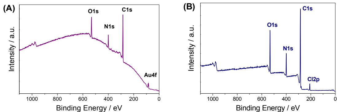
Figure 5: XPS survey spectra obtained from films electrogenerated in 0.15 M Py + 0.2 M \text{K}_2\text{HPO}_4 + 10^{-4} M (A) or 5 \cdot 10^{-3} M (B) \text{LiClO}_4 , at 0.78 V/SCE for 600 seconds, on Au/mica substrates.
