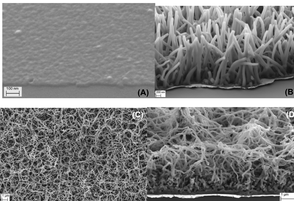
Figure 2: SEM images from PPy films electrogenerated in (A) 10^{-4} M \text{LiClO}_4 + 0.2 M \text{K}_2\text{HPO}_4 + 0.15 M Py ; (B) 10^{-3} M \text{LiClO}_4 + 0.2 M \text{K}_2\text{HPO}_4 + 0.15 M Py ; (C,D) 5 \cdot 10^{-2} M \text{LiClO}_4 + 0.2 M \text{K}_2\text{HPO}_4 + 0.15 M Py at 0.78 V/SCE for 600 s (A, C, D) or 1000 s (B). (A, B, D) cross section, \theta = 65^\circ . (C) Top view. Substrates: (A) a-CNx, (B, C, D) Au/mica. Scale bars: (A) 100 nm, (B) 200 nm, (C, D) 1 \mu\text{m} .
