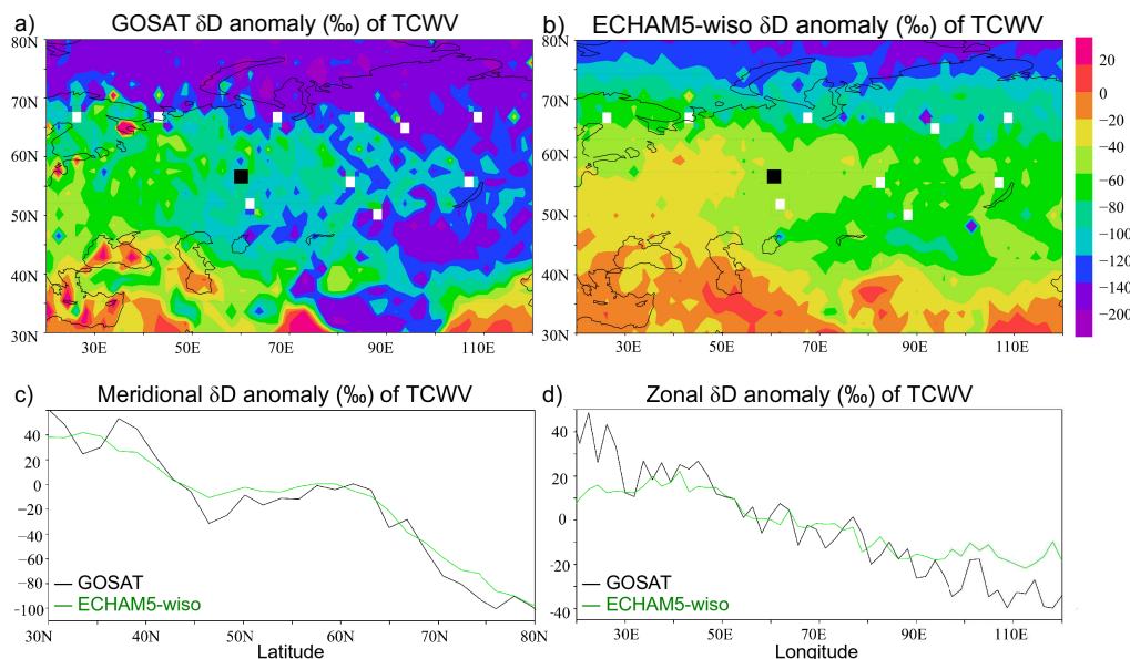
Figure 2. Distribution of annual-mean \delta D in total column water vapour, (a) as observed by the GOSAT satellite, (b) as simulated by ECHAM, after collocation with GOSAT observations and convolution with the corresponding averaging kernels. In (a) and (b) the global average of \delta D has been subtracted to highlight spatial patterns, and the black squares indicate the location of Kouroukva Observatory; white squares are grid cells with low-quality observations. (c) Meridional transects of observed (black) and simulated (green) \delta D averaged over the longitude band 50\text{--}70^\circ\text{E} around Kouroukva. The annual-mean \delta D value averaged over the area 30\text{--}80^\circ\text{N} , 50\text{--}70^\circ\text{E} has been subtracted to highlight the meridional variations. (d) Zonal transects of observed (black) and simulated (green) \delta D averaged over the latitude band 50\text{--}64^\circ\text{N} around Kouroukva. The annual-mean \delta D value averaged over the area 50\text{--}64^\circ\text{N} , 20\text{--}120^\circ\text{E} has been subtracted to highlight the zonal variations.
