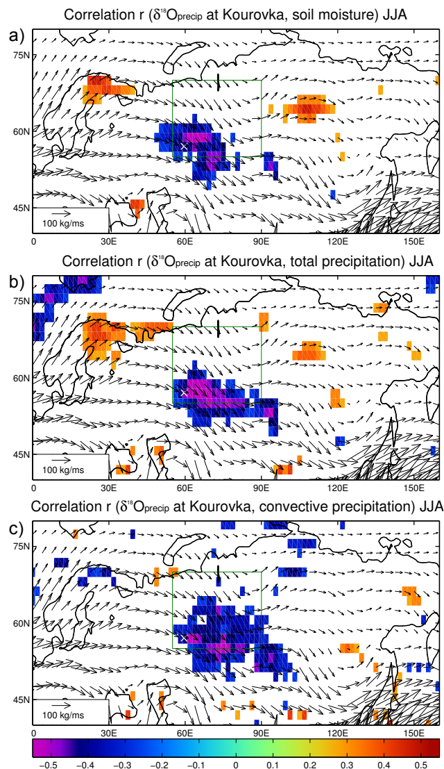
Figure 11. One-point correlation map showing the correlation between \delta^{18}\text{O} in precipitation at Kourvka during summer (JJA) with (a) soil moisture, (b) total precipitation, and (c) convective precipitation. Also shown is the average atmospheric moisture transport during JJA (vectors; only every second vector is drawn). The green box indicates western Siberia and the position of Kourvka is marked by a white cross. The correlation period is 1960–2010. Statistically insignificant areas (where p \geq 0.05 applying a t test) are blanked. See also Table 3 for numbers.
