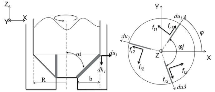
Fig. 11: The reaming model principle
