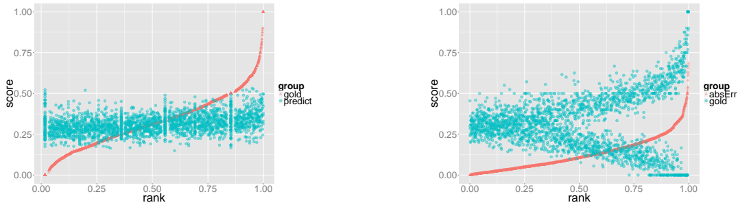
(a) Gold scores as reference. Sentences are sorted by their gold score; the X axis gives their corresponding rank; the predicted score of a sentence is plotted on the same abscissa, thus showing both the gold (in red) and predicted score (in blue) of the sentence on the Y axis. The predicted scores which appear on the same vertical line correspond to different sentences which have the same (or very close) gold scores.
