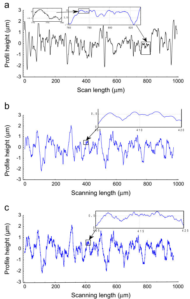
Fig. 15. (a) Profile of a pure Aluminium sheet surface polished with paper grade 500 with a 10\ \mu\text{m} stylus tip curvature. (b) Simulation of the scanning of the profile c with a 10\ \mu\text{m} stylus tip curvature. (c) Simulation of profile a by stochastic circle function.
