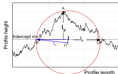
Fig. 1. Definition of l_x and l_y used to calculate the local curvature radius r_c(l_x) .
