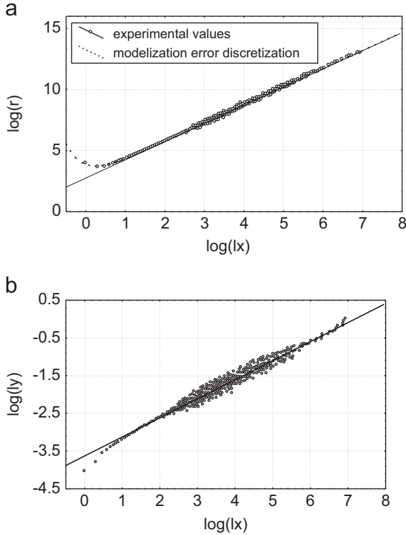
Fig. 5. Evolution of the curvature radius \log(r) of the profile shown in Fig. 3a, estimated at a l_x value versus the \log l_x value (a). The thin line corresponds to the equation \log r_c(l_x) = 2.756 \pm 0.01 + 1.488 \pm 0.004 \log l_x and the dashed one to the corrected method with \log r_c(l_x) = 2.732 \pm 0.01 + 1.494 \pm 0.003 \log l_x + 1.14 \pm 0.1 / (l_x - 1) (where n_x is the number of d_x intervals used to calculate l_x ). The graph (b) represents the evolution of the height curvature radii \log l_y(l_x) versus the \log l_x value.
