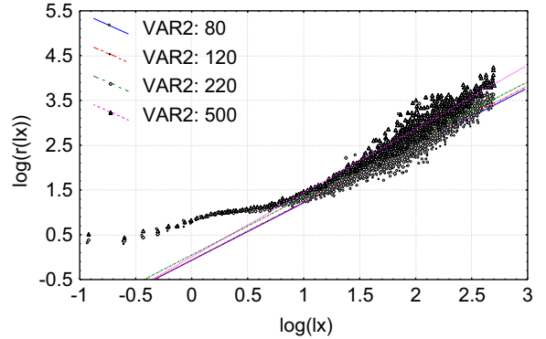
Fig. 14. Evolution of the curvature radius \log r_c(l_x) versus \log l_x for pure Aluminium sheet surface polished with different paper grades 80, 120, 220 and 500 ( l_x and r(l_x) in \mu\text{m} ).
