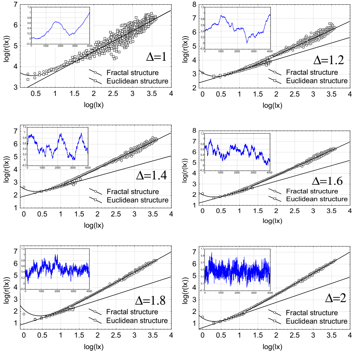
Fig. B2. Evolution of the fractal curvature radius \log r(l_x) and Euclidean curvature radius \log \tilde{r}(l_x) versus \log l_x for different fractional Brownian curves (fractal dimension 1, 1.2, 1.4, 1.6, 1.8, 2) with their associated profiles.
