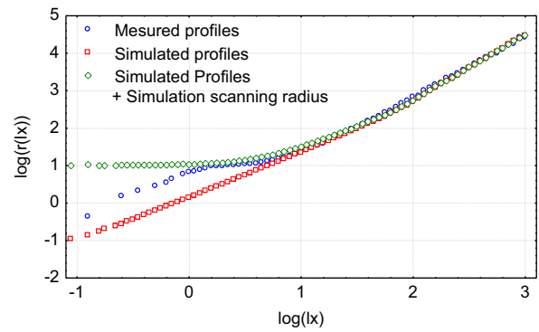
Fig. 16. Evolution of the curvature radius \log r(l_x) versus \log l_x for profile shown in Fig. 15a, Fig. 15b and Fig. 15c ( l_x and r(l_x) in \mu\text{m} ).
