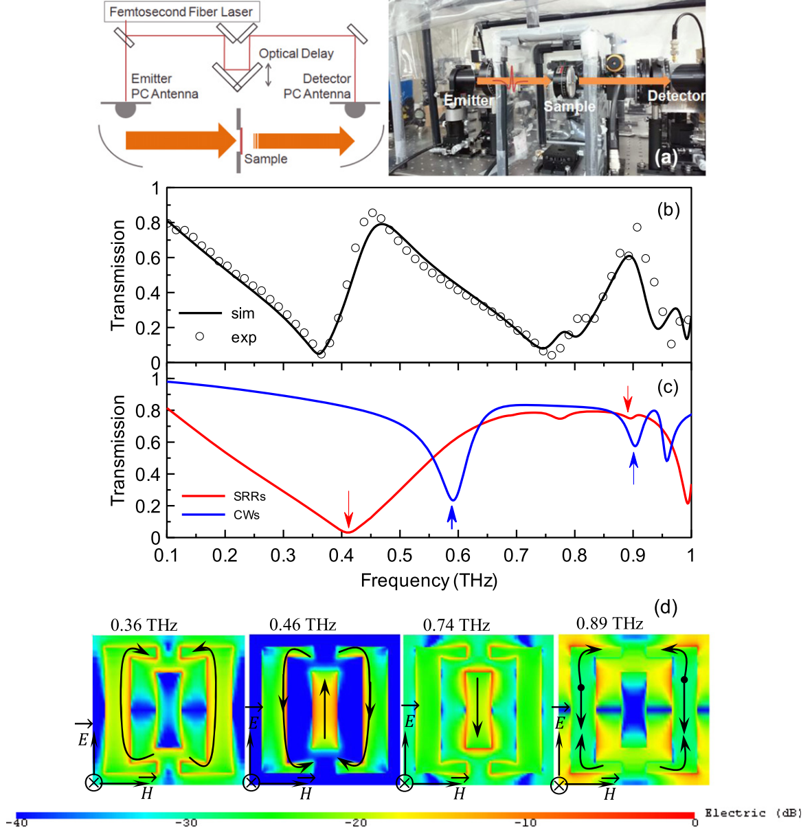
Figure 2. (a) Schematic diagram and photograph of the THz TDS setup used for experimental measurements. (b) Simulated (solid line) and measured (hollow circles) transmission spectrum of the investigated metamaterial. (c) Amplitude of the transmission of SRRs and CWs in the case of TM polarized incidence plane wave ( E \parallel \text{CWs} ). (d) Electric field amplitudes and surface current directions when driven by the incident field (denoted by black arrows for greater clarity) from left to right at the lower frequency resonance of 0.36 THz, at the transparency peak of 0.46 THz, at the higher frequency resonance of 0.74 THz and at the transparency peak of 0.89 THz.
