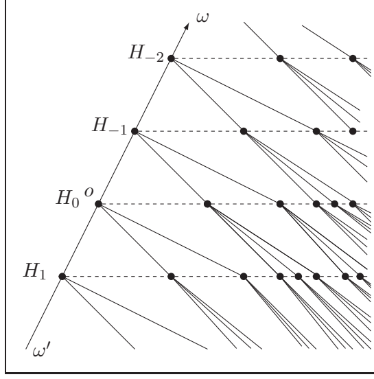
FIGURE 1. Example \mathbb{T}_3
