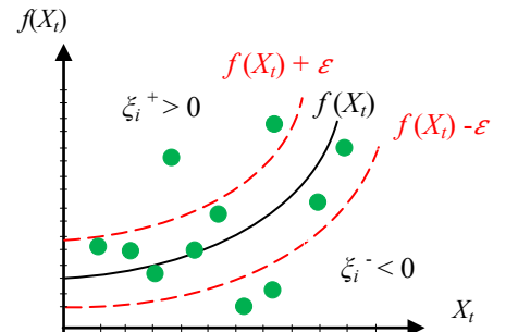
Fig. 7. Regression with \varepsilon -insensitive tube.
