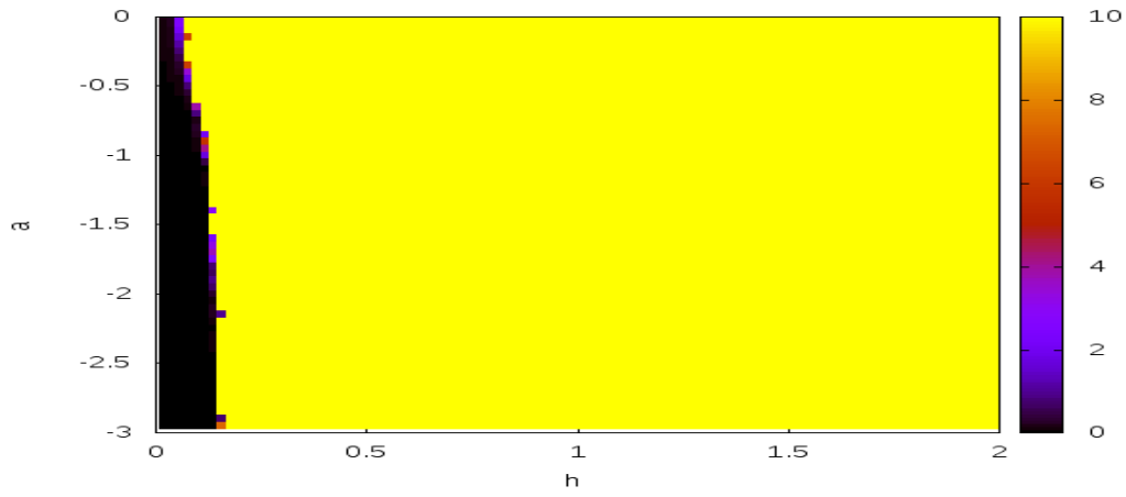
FIGURE 6. Empirical stability of pseudo-explicit Euler scheme
