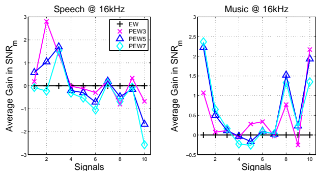
Fig. 3. Influence of the neighborhood on deconvolving performance. The 10 different speech (left) and music signals (right) are displayed on the x-axis. The average gain (over clipping levels 0.1, 0.2, ..., 0.9) of SNR_{miss} with regard to the baseline set by the EW operator is displayed on the y-axis.
