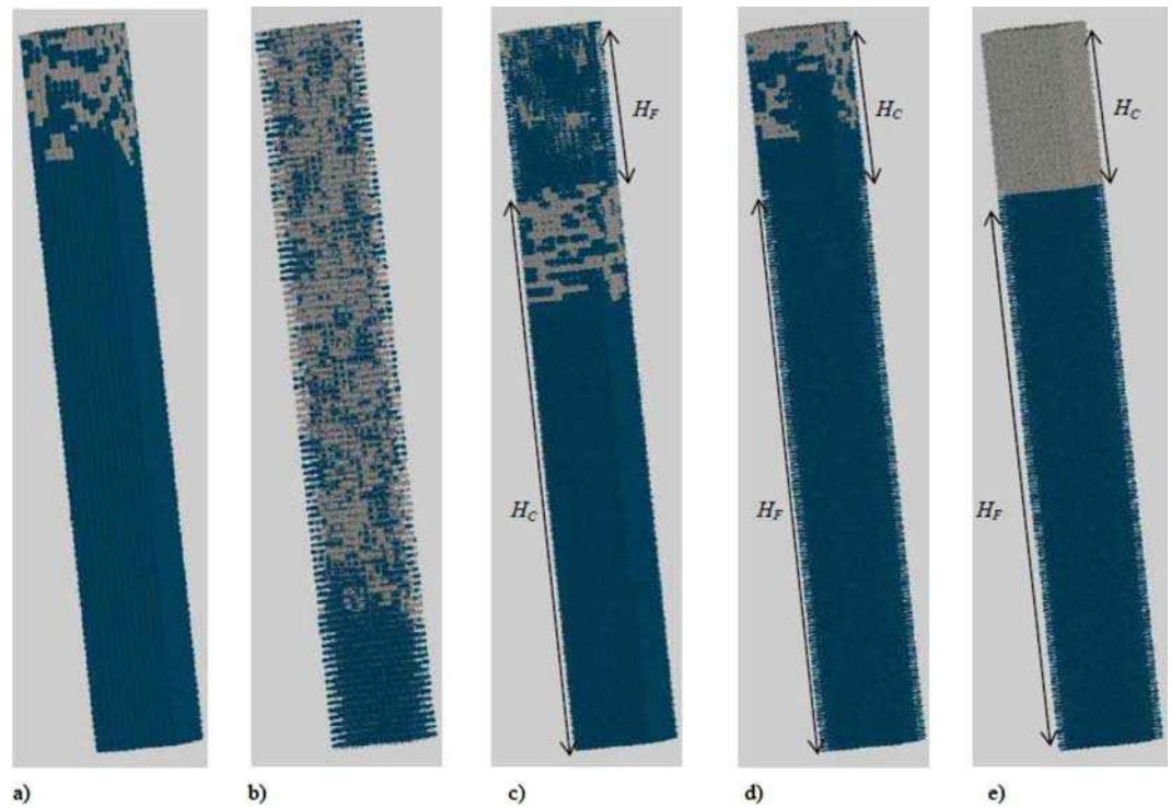
Figure 1. Examples of phase distribution in a column of square cross section and of total height H obtained using pore network simulations (the liquid phase is in blue, the gas phase in gray): (a) coarse porous medium at the end of S1 ; (b) fine porous medium at the end of S1 ; (c) fine layer (thickness H_F ) over coarse medium when the liquid phase in the coarse region ceases to be hydraulically connected to the top fine layer; (d) coarse layer (thickness H_C ) over fine medium at the end of S1 ; (e) coarse layer over fine medium when the coarse layer is entirely dry and the fine layer begins to dry. Evaporation (gas invasion) is from top surface only. The size of network is 16 \times 16 \times 100 . The thickness of the top layer in Figures 1(c)–1(e) is 24.
