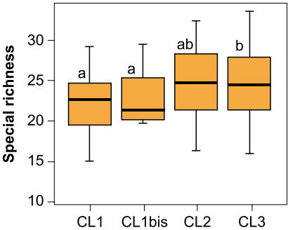
Figure 5.9: Box plots showing species richness (mean SR.m -2 ; n=5 replicates) variations in the four clusters from the CA. see text for details. Boxes sharing the same letter are not statistically different (P < 0.05, Tukey's HSD comparing all clusters).
