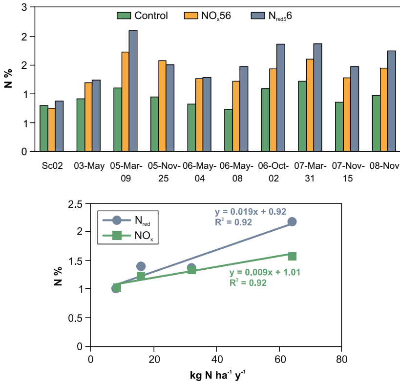
Figure 5.21: a) Nitrogen concentrations (per cent dry wt) in Sphagnum capillifolium treated with 56 kg N ha -1 of nitrate (NO x ) or ammonium (Nre) and the control between 2002 pre treatment and the end of 2008; and b) Pleurozium schreberi in March 2009 in relation to N dose in precipitation
