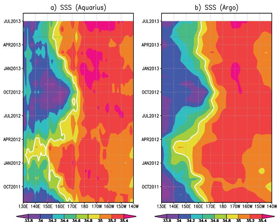
Figure 6. Time-longitude distribution of sea surface salinity along the 3^{\circ}\text{S} – 3^{\circ}\text{N} equatorial band in the western central Pacific from (a) Aquarius and (b) Argo for the period August 2011 to July 2013. The white lines are the 34.8 psu isohalines representing the SSS front.
