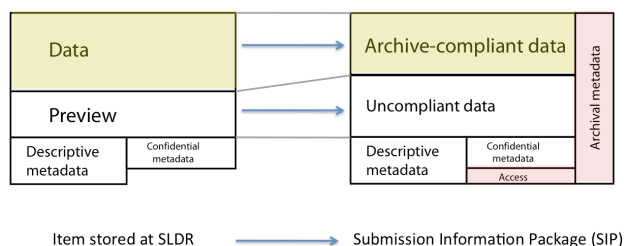
Figure 3: The making of a submission information package on SLDR
