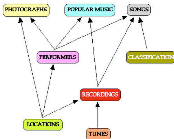
Figure 2: The relational database of grindmill songs at CCRSS in 1996.
