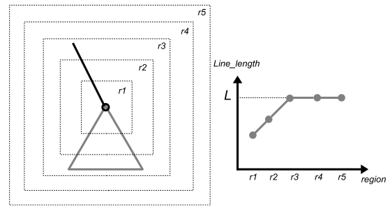
Fig. 12 Multi-scale Detection.
