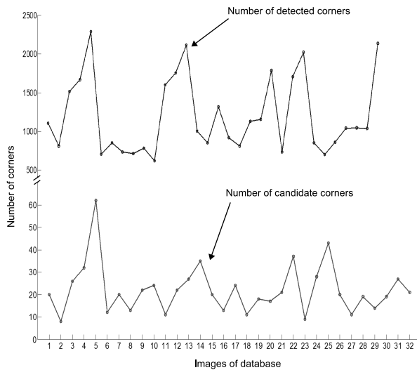
Fig. 6 Results of corner coding on 32 images of Grigorescu's database of traffic signs [15]. The top curve represents the number of detected corners with the Harris detector. The bottom curve represents the number of selected corners with the proposed corner coding method
