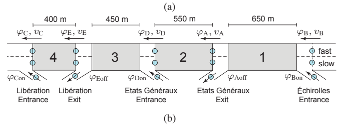
Fig. 7. (a) The section of Grenoble south ring considered in our experimental study (image source: Google Maps); (b) The section has been subdivided into four cells whose length ranges from 400 to 650 meters: the disks indicate pairs of magnetometers spaced 4.5 m apart.
