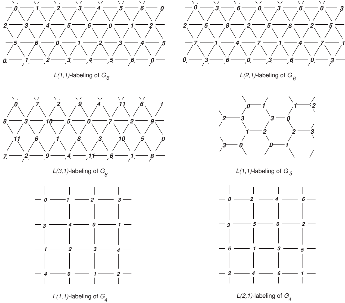
Fig. 3: L(1, 1) -, L(2, 1) - and L(3, 1) -labelings of regular grids.
