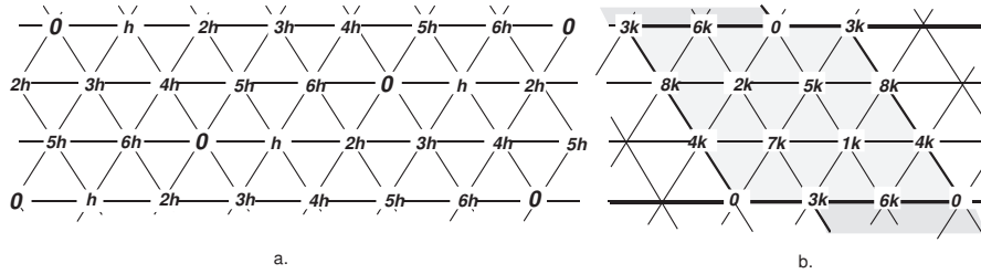
Fig. 5: Feasible labelings of a cellular graph when a. k \leq h \leq \frac{4}{3}k and when b. \frac{4}{3}k \leq h \leq 2k .
