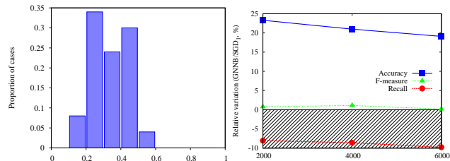
Fig. 8. Left: frequency of cases among classes for the proportion of examples used per class by GNNB; Right: GNNB* ( k = 200 ) vs SGD 1 (conventions follow Fig. 7).
