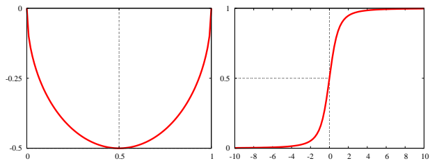
Fig. 1. Plot of permissible \phi of row D in Table 1 (left) and its matching posterior estimate \hat{p}_{\phi,h} as a function of h \in \mathbb{R} (right, see text).
