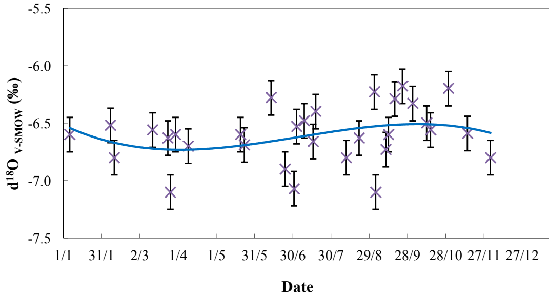
Figure 4. Variation of the \delta^{18}\text{O} values of the reference groundwater well near Verdun sur Garonne (between 1997 and 2003) over the season. The solid line represents the polynomial regression line.
