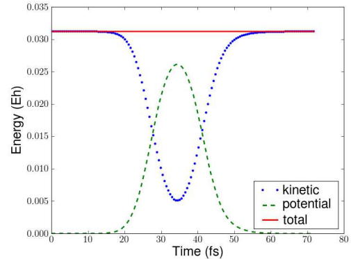
FIG. 4. Evolution of the energy during the propagation
