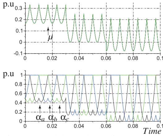
Figure 10: \mu and duty cycle waveforms, taken for reduced switching losses.
