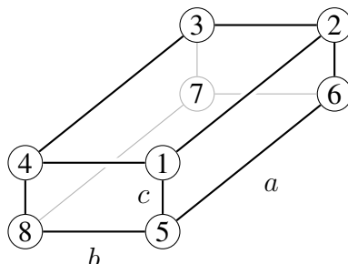
Figure 2. Rectangular parallelepiped.
