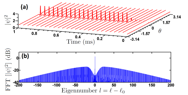
FIG. 2: Temporal cavity soliton with \alpha = 1.7 , \beta = -0.002 and F = 1.22 . The intracavity pump is |\psi_0|^2 = 0.95 , so that it is below threshold. (a) Cavity soliton formation. (b) FFT of the soliton, corresponding to a wide-span, low-threshold Kerr frequency comb.
