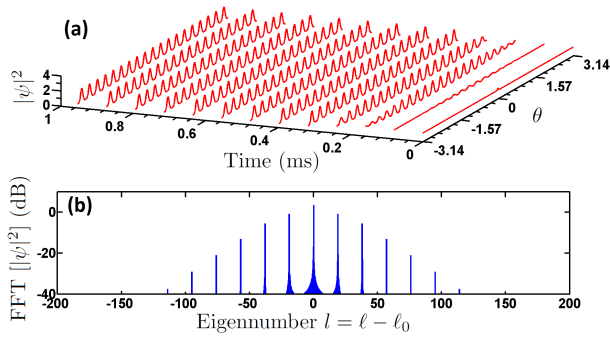
FIG. 1: Multiple-FSR comb with \alpha = 0 , \beta = -0.0125 and F = 1.71 . The intracavity pump is |\psi_0|^2 = 1.2 , so that it is above threshold |\psi|_{\text{th}}^2 = 1 . The parameters correspond to Fig. 10b in ref. [6]. (a) Time-domain dynamics that consists of 19 smooth pulses (“roll” Turing pattern solution). (b) FFT of the roll solution, corresponding to an order 19 multiple-FSR comb.
