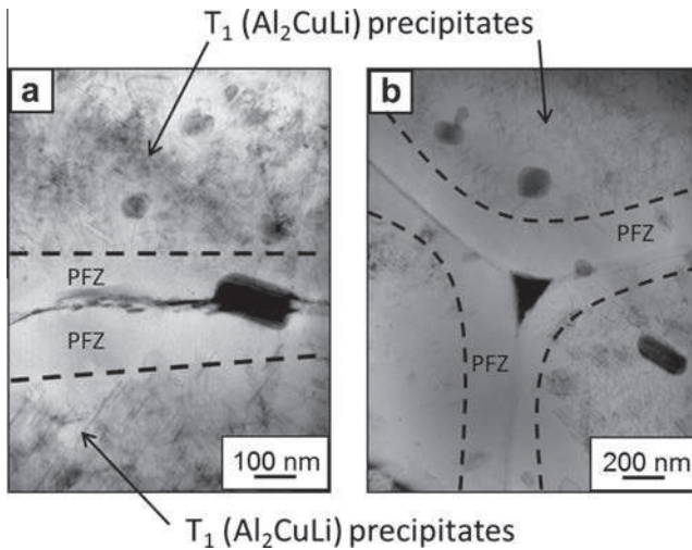
Fig. 6. TEM observations of the PWHT nugget of the AA 2050 FSW joint in the bands susceptible to be corroded: (a) intergranular precipitates and Precipitate Free Zone and (b) similar observations in another zone.
