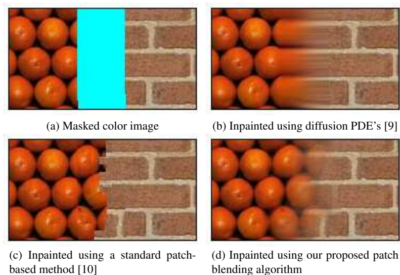
Fig. 4: Illustrating the advantage of patch blending on a synthetic case.
