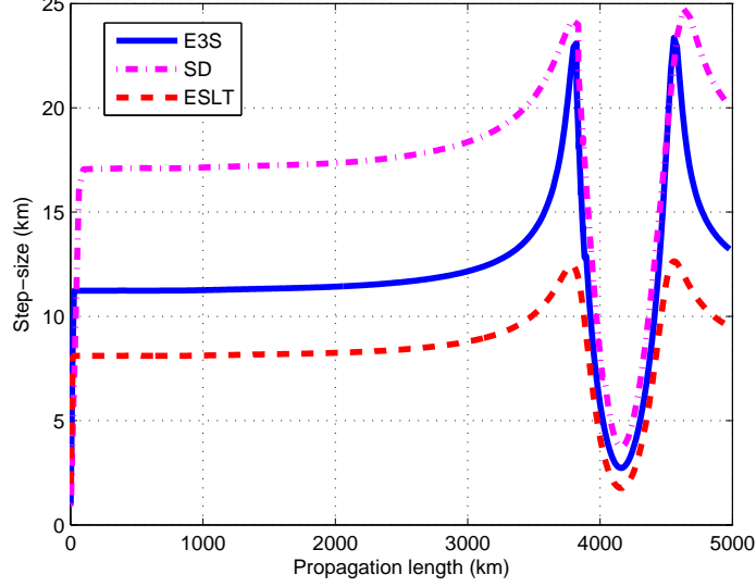
Figure 2: Evolution of the step-size along the fiber for the E3S, SD and ESLT methods for soliton collision.
