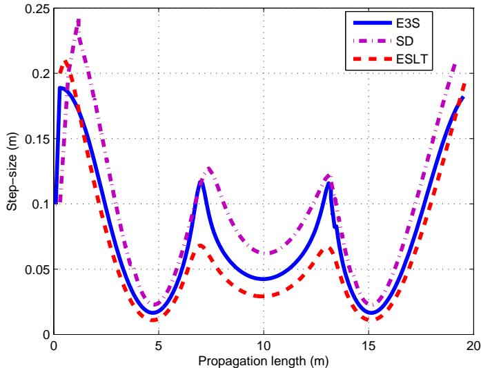
Figure 1: Evolution of the step-size along the fiber for the E3S, SD and ESLT methods for a 3rd order soliton with a tolerance set to 10^{-3} .
