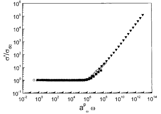
Figure 6. Master curve as a function of [\sigma'(\omega,T)/\sigma_{dc}] as a function of a_\omega^p \omega for p \geq p_c : (▼) 0.3, (◇) 0.4, (■) 0.6, (○) 0.8, (▲) 1.5, and (▽) 2.5 wt %.
