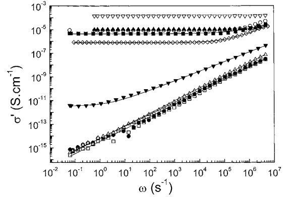
Figure 1. Frequency dependence of the real part \sigma' of the complex conductivity for different carbon nanotubes weight fraction p at 20 °C: (□) 0, (●) 0.04, (△) 0.2, (▼) 0.3, (◇) 0.4, (■) 0.6, (○) 0.8, (▲) 1.5, and (▽) 2.5 wt %. The solid lines are fits to eq 1.
