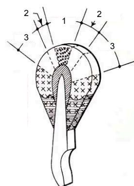
(c) Hammer head needling zones. Zone 1 : weak - light needling for piano dynamics. Zone 2 : medium - deep needling for mezzo-forte dynamics. Zone 3 : heavy - deep needling for forte dynamics. From [20].
