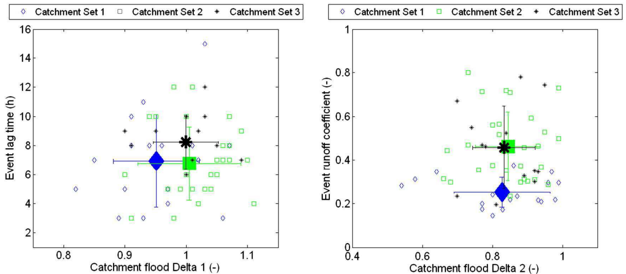
Fig. 10. (left) Event lag time related to Event catchment flood \Delta_1 ; (right) Event runoff coefficient related to catchment flood \Delta_2 .
