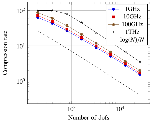
Figure 2: Compression rate vs the number of degrees of freedom (dofs).
