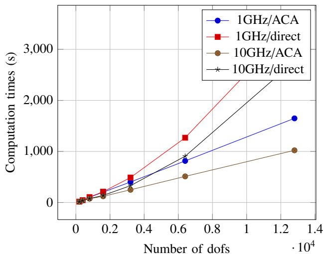
Figure 3: Computation times.
