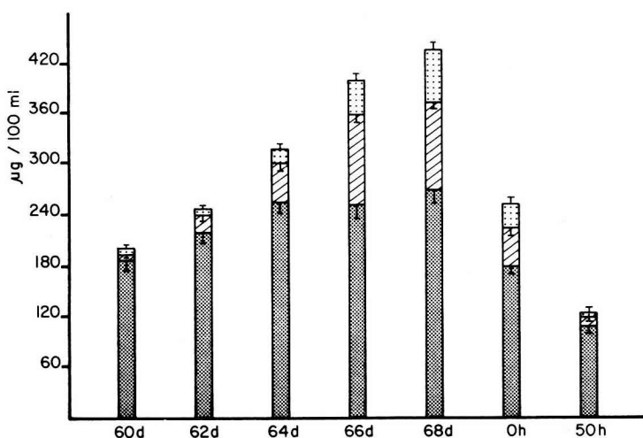
FIG. 2. — Development of free ( ), albumin-bound ( )
