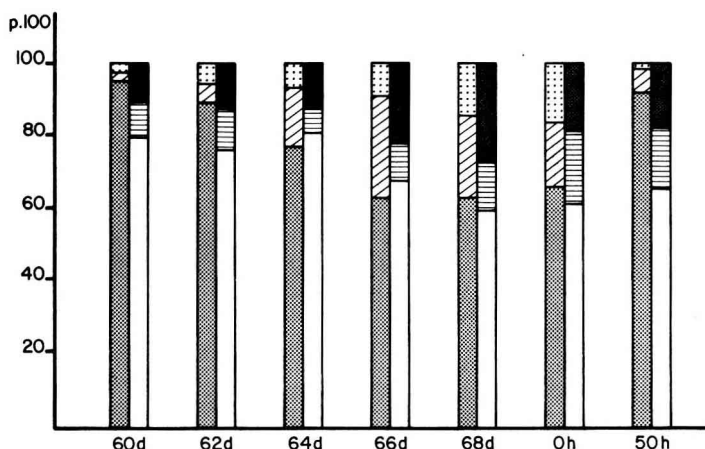
FIG. 3. — Changes in percentage of free, albumin-bound, and transcortin-bound cortisol in mother, foetal and newborn guinea-pigs during the perinatal period. Mother : free (□) ; albumin-bound (▨) ; transcortin-bound (▩). Foetal and newborn : free (■) ; albumin-bound (▤) ; transcortin-bound (open bars).
