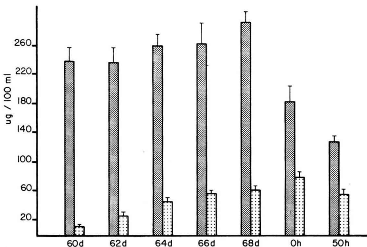
FIG. 1. — Changes in transcortin binding capacity for cortisol in maternal (▨ ; n = 6-10 ) and foetal and neonatal (▤ ; n = 6 ) guinea-pigs during the perinatal period.
