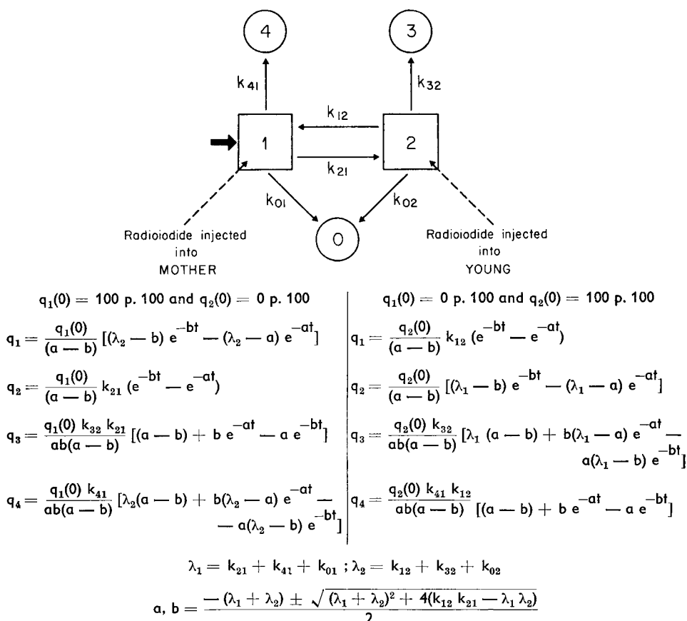
FIG. 1. — Theoretical and mathematical model for non-hormonal iodine metabolism in rat family on day 10 post-partum. Thick arrow indicates maternal dietary iodine uptake; k symbols with subscripts are rate constants of iodine transfer to compartment 1 from compartment 2, to compartment 2 from compartment 1, etc.; q symbols with subscripts show radioactivity of the compartments at a given time after radioiodide injection into the dam (left) or the pups (right); q_1(0) and q_2(0) are q_1 and q_2 at zero time.
