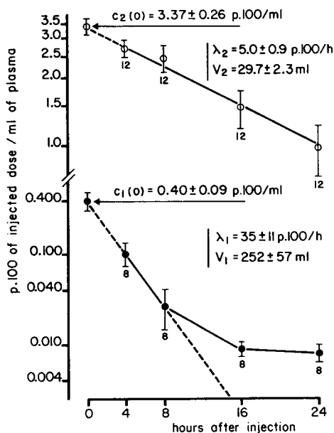
FIG. 3. — Plasma radioiodide clearance curves after injection of labelled I^- . Upper curve : plasma radioiodide of injected dam minus non-injected pups in the same litter. Lower curve : plasma radioiodide in injected dam. c_1(0) and c_2(0) = extrapolated concentrations at zero time ; rate constant \lambda_1 is estimated from the first two points of the dam's curve, and \lambda_2 from the total pup curve ; V_1 and V_2 = distribution volumes of unlabelled iodide in the dam and pups, respectively. For other explanations see text and figure 2.
