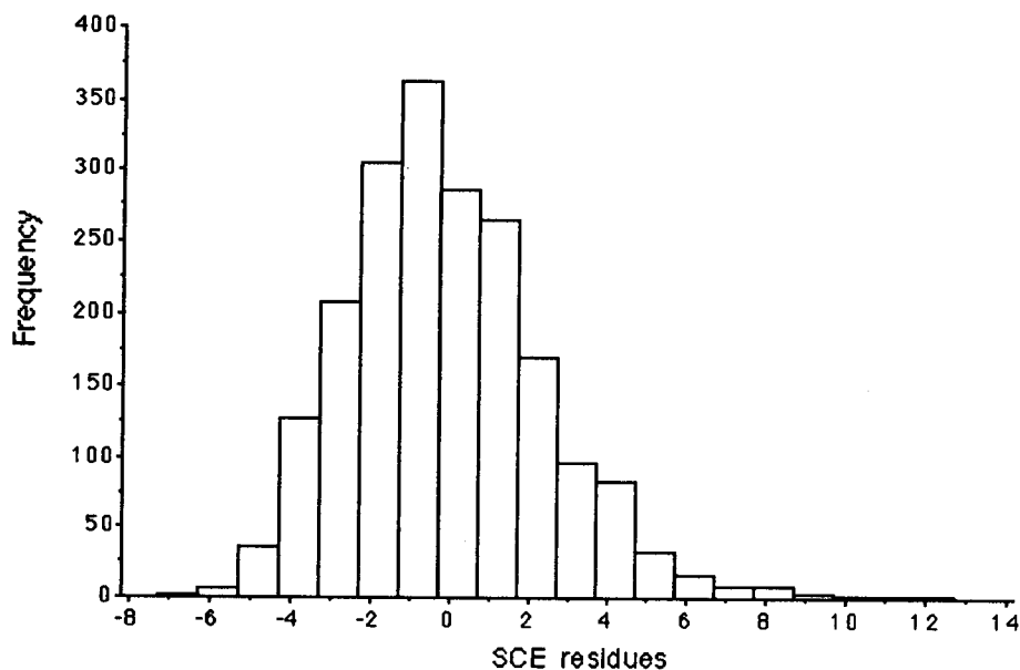
Fig 1. Histogram of the frequency distribution of SCE residuals.
