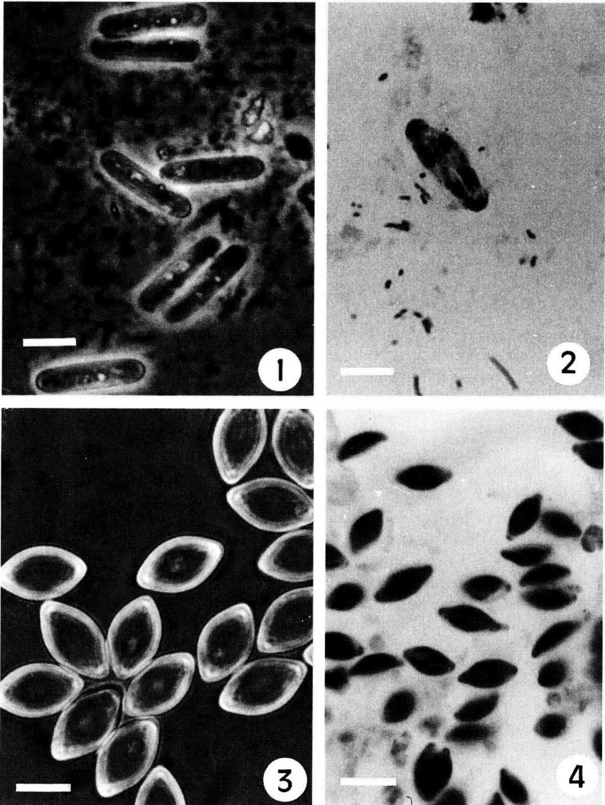
Figs 1–2. Apicystis bombi . 1. Fresh oocysts from tissues of B terrestris (bar = 8 \mu m). 2. Fixed and stained young oocysts from A mellifera with four visible uninucleate sporozoites (bar = 7 \mu m). Figs 3–4. Mattesia dispora . 3. Fresh oocysts from tissues of Anagasta künniella (bar = 7 \mu m). 4. Fixed and stained oocysts (bar = 11 \mu m).
