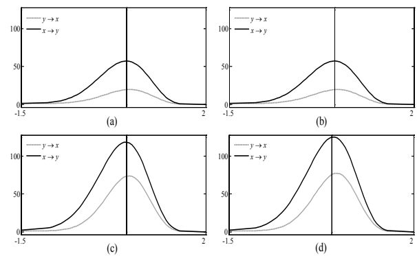
Fig. 3. Means of TE values in the second linear model. (a) The orders are estimated by AIC. (b) The orders are estimated by BIC. (c) The orders are estimated by gAIC. (d) The orders are estimated by gBIC. Solid line: flow direction x \rightarrow y , dotted line: flow direction y \rightarrow x .
