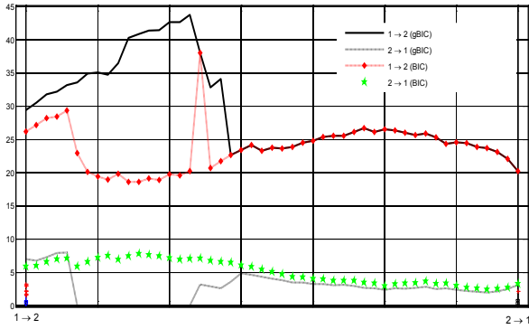
Fig. 6. Results on TE with the orders estimated by gBIC and BIC for 2 real iEEG signals. Signal 1 corresponds to a signal recorded in m-EC and signal 2 to a signal recorded in PRC.
