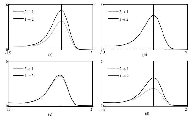
Fig. 4. Means of TE values in physiology-based models where the models' orders are estimated by BIC and gBIC. (a) Populations 1 and 2 are unidirectionally coupled and the orders are estimated by BIC. (b) Populations 1 and 2 are unidirectionally coupled and the orders are estimated by gBIC. (c) Populations 1 and 2 are bidirectionally coupled and the orders are estimated by BIC. (d) Populations 1 and 2 are bidirectionally coupled and the orders are estimated by gBIC.
