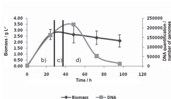
Figure 5 DNA quantification of G. candidum in pure culture. Growth exponential phase, b); transition phase, c); stationary/decay phase, d).
