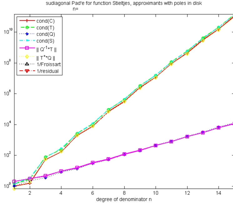
Figure 1: Condition numbers related to the Stieltjes function f_1 .
