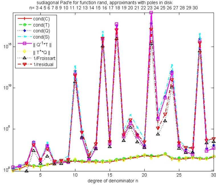
Figure 3: Condition numbers related to the random function f_3 .
