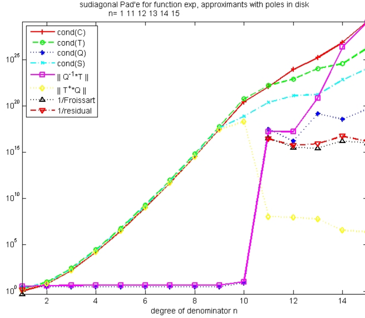
Figure 2: Condition numbers related to the exponential function f_2 .
