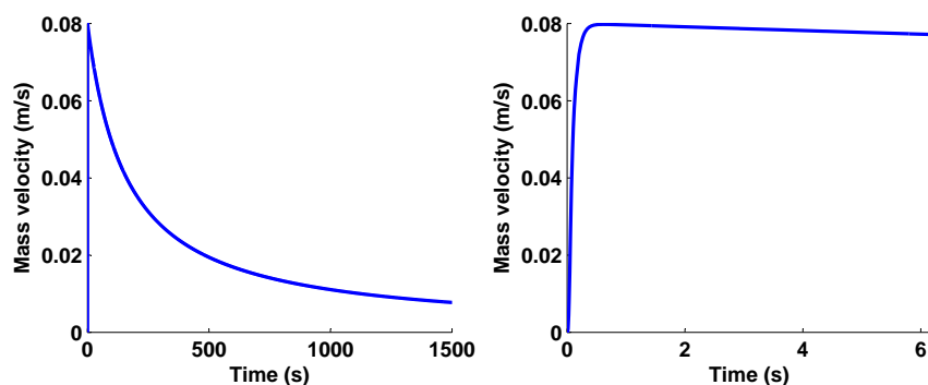
Fig. 17: Time response of the system under a linear degradation (left figure) and zoom on the first seconds (right figure).
