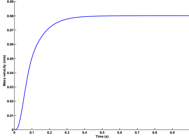
Fig. 10: Step response of the mechatronic system.
